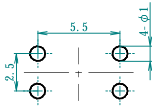
Hole Layout Recommended P.C Board thickness t=1.6
