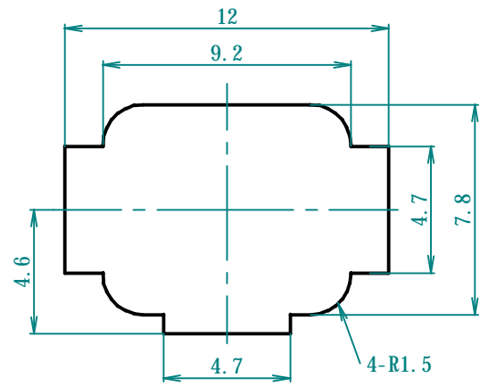
Mating Hole Recommended Panel thickness t1.6
