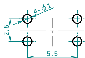
Hole Layout Recommended P.C Board thickness t1.6mm
