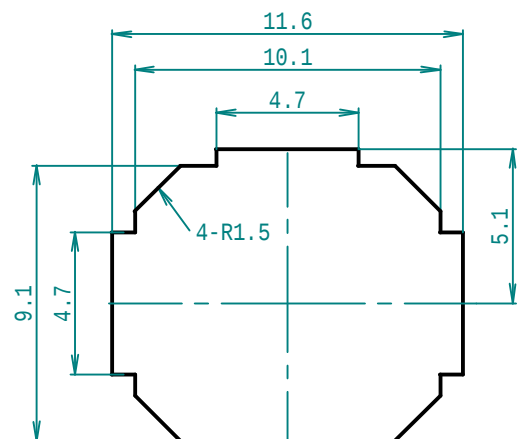
Mounting Hole Recommended Panel thickness t1.6mm
